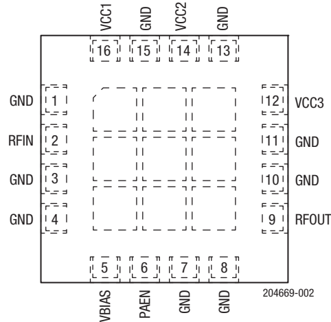
Figure 2. SKY66397-12 Pinout (Top View)
