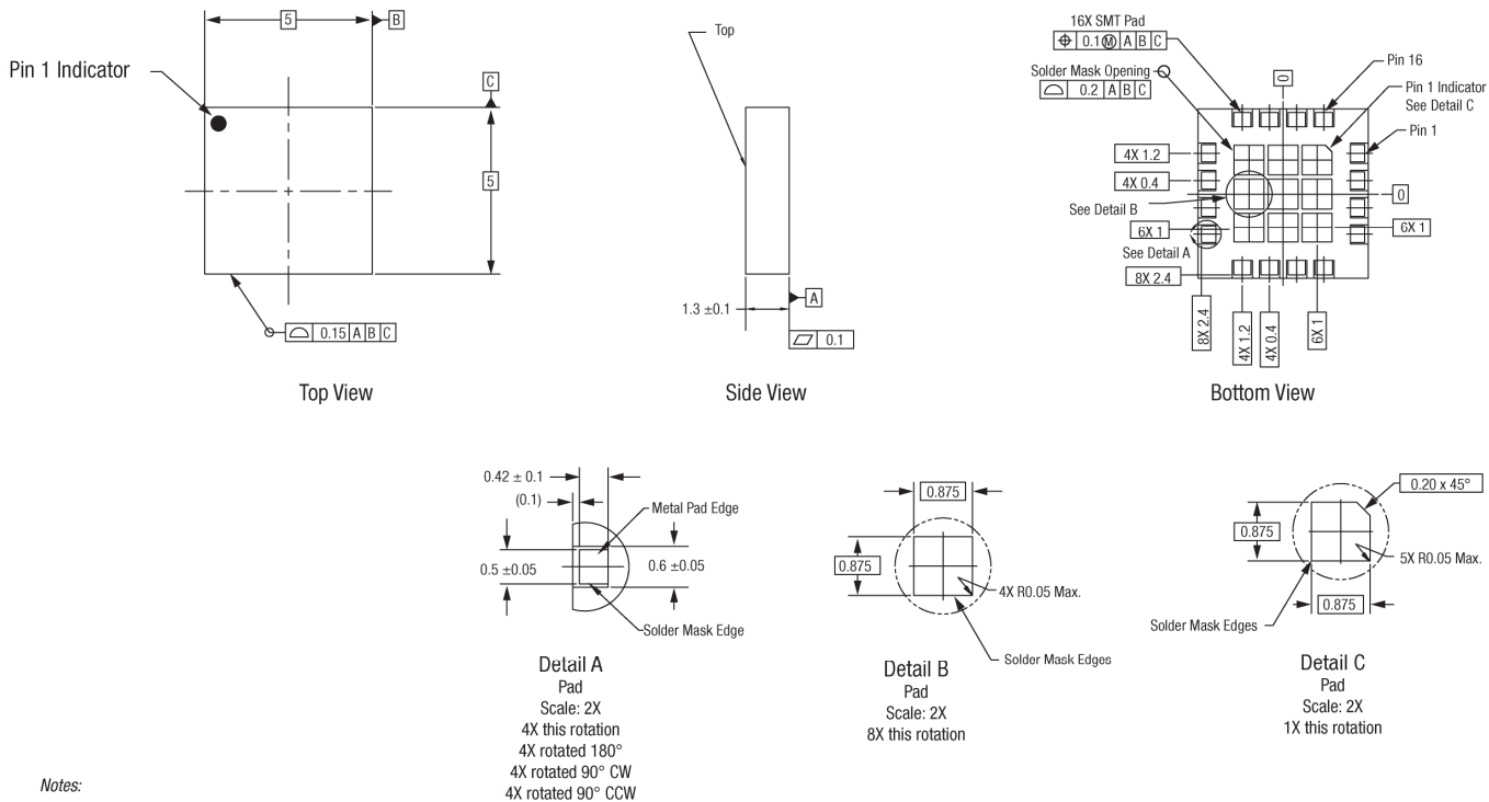
Figure 23. SKY66397-23 Package Dimensions
