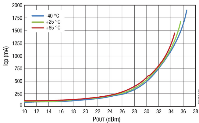
Figure 10. Iop vs POUT Across Temperature
